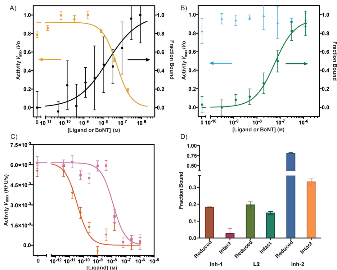
Figure 1. Characterization of ligand binding and inhibition in vitro. A) Inhibition curve (left axis) and fluorescence polarization binding curve (right axis) of Inh-1. An IC 50 value of inhibition of 70 \pm 10 nM and a K_D value of 68 \pm 29 nM were obtained by Hill curve fitting. B) Inhibition curve (left axis) and fluorescence polarization binding curve (right axis) of compound L2. No inhibition was observed, and a K_D value of 78 \pm 8 nM was determined. C) Inhibition curves comparing Inh-1 (pink) to Inh-2 (red). IC 50 values of 60 \pm 11 nM and 165 \pm 15 pM, respectively, were observed. D) Single-point ELISA binding data of compounds to 50 nm of the reduced (available active site) and intact (occluded by belt) BoNT/A holotoxins. Error bars indicate standard deviation of replicates.
